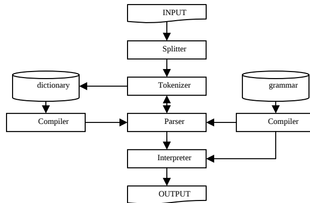
Fig. 1 HERMETO's architecture
